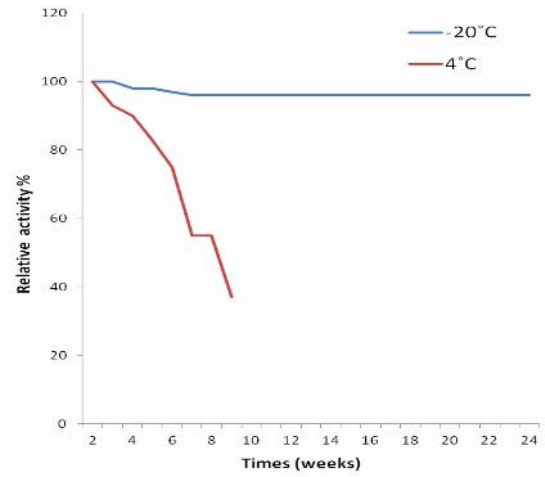
Figure 5. Effect of storage temperature on \alpha -amylase activity from Bacillus licheniformis SUDK2
