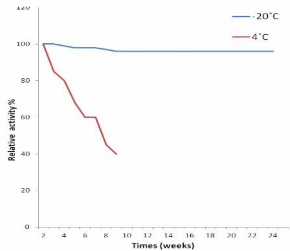
Figure 7. Effect of storage temperature on \alpha -amylase activity from \alpha -amylase activity from Bacillus licheniformis SUDO
