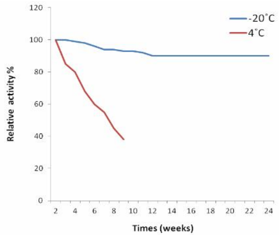
Figure 6. Effect of storage temperature on \alpha -amylase activity from \alpha -amylase activity from Bacillus licheniformis SUDK4
