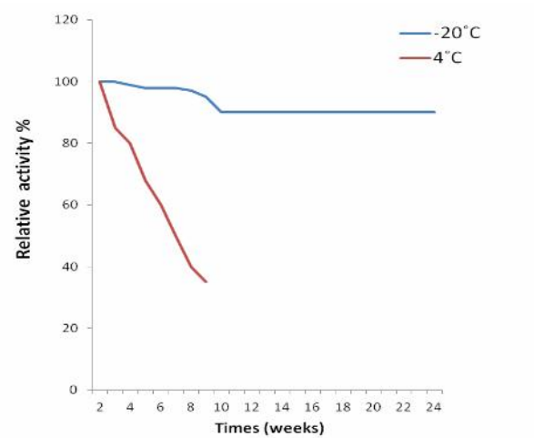
Figure 4. Effect of storage temperature on \alpha -amylase activity from \alpha -amylase activity from Bacillus licheniformis SUDK1
