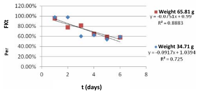
Figure 2. The gradient relationships between the rate of 137 Cs release and exposure time
