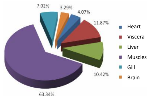
Figure 5. The distribution of 137 Cs accumulation inside the body of Cromileptes altivelis .
