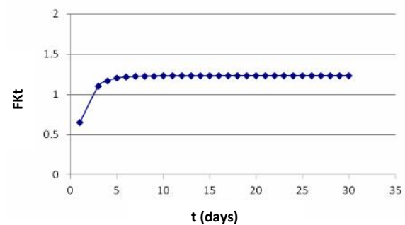
Figure 3. The estimation of CF ss of 137 Cs in Cromileptes altivelis with average body mass of 65.8 g
